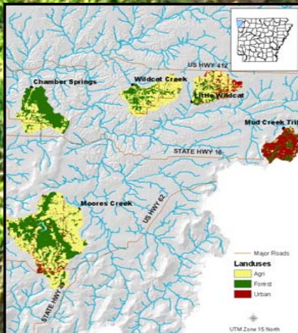
Figure 1: Land use/land classification of 5 stream sites within the Illinois River Watershed.
